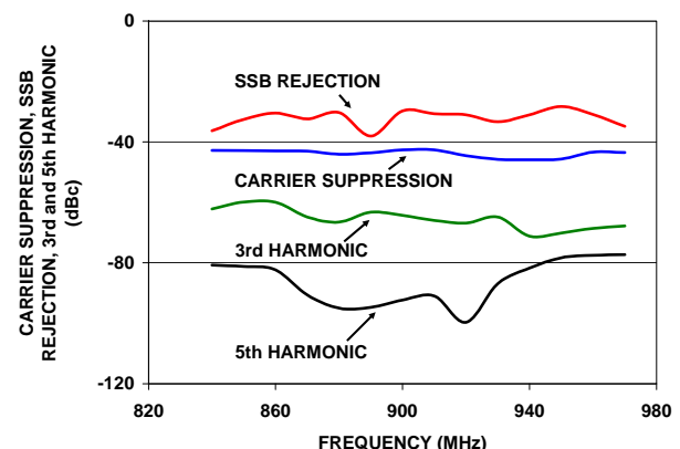
Carrier Suppression, SSB Rejection, 3rd and 5th Harmonic Suppression: V_{CC} = 3.3\text{V} , P_{LO} = +2\text{ dBm}
